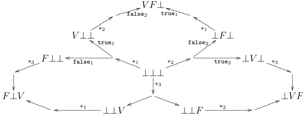
Fig. 1. A fragment of the extensional data structure !\mathbb{B} \otimes !\mathbb{B} \otimes !\mathbb{B} .
