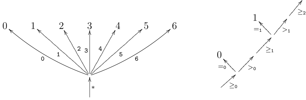
Fig. 3. The flat natural number eds \mathbb{N}_{\text{flat}} vs. the lazy natural number eds \mathbb{N}_{\text{lazy}} .
