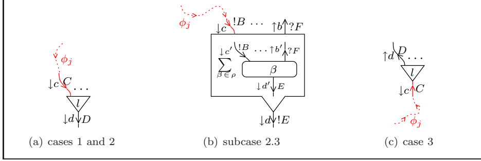
Figure 11: main cases of the proof of Lemma 3.2.
