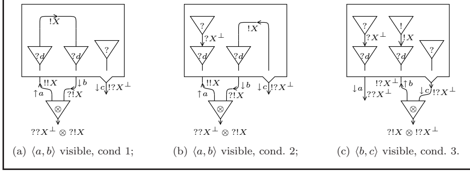
Figure 5: examples of visible cycles (Definition 2.5).
