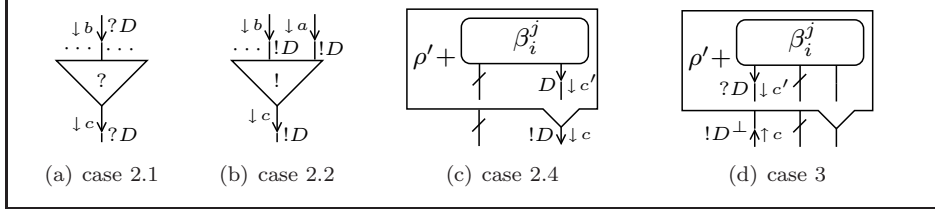
Figure 15: main cases in the proof of Lemma 4.4.
