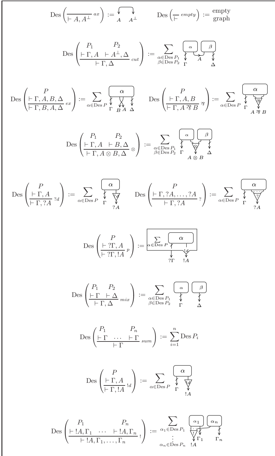
Figure 3: desequentialization of the proofs of the DiLL sequent calculus; as for the 0-cocontraction, we mean that its desequentialization is the simple net consisting of a unique !-cell.
