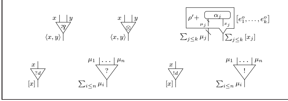
Figure 9: conditions required to experiments. Experiments are pictured as wire/box's labelling. In case of a box !\rho , we set \rho' := \rho - \alpha_j , for every \alpha_j \in \rho .
