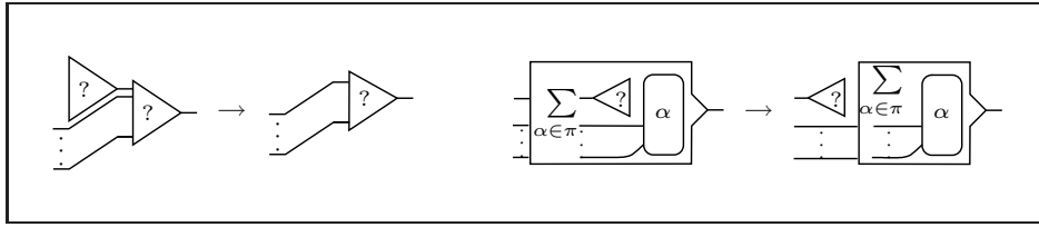
Figure 8: elementary steps of the elimination of weak wires: in the step pictured at left, the contraction in the reduct which comes out to have 2 ports is a convention to denote a single connecting wire.
