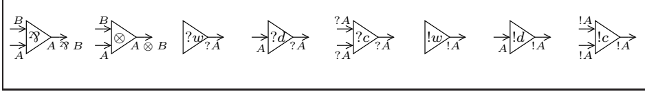
Fig. 2: cells for differential interaction nets, together with their typing rules.
