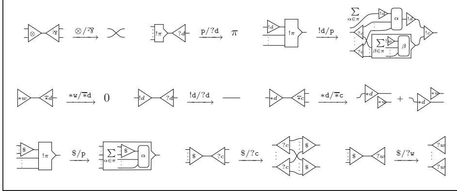
Fig. 4: elementary reduction steps (ers) for differential nets, where * (resp. \bar{*} ) is ? (resp. ! ) or ! (resp. ? ), and \$ is !w , or !c , or !\pi . In the !w/?w ers the contractum is the empty graph.
