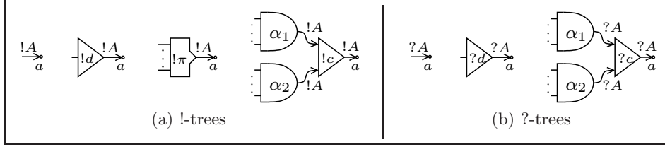
Fig. 7: inductive definition of !/?-trees.
