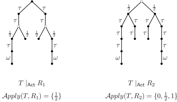
Fig. 5. Counterexample: action prefix does not distribute over probabilistic choice
