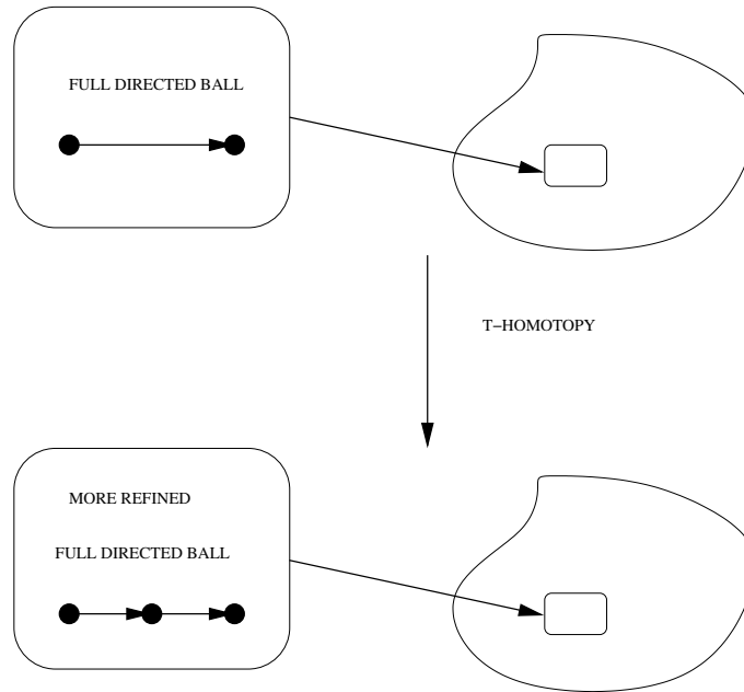
FIGURE 3. Replacement of a full directed ball by a more refined one
