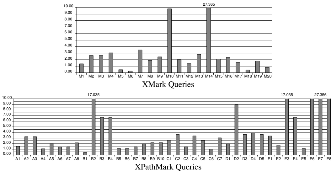
Fig. 7. Pruning ratio (% of the original file size) for XMark and XPathMark queries
