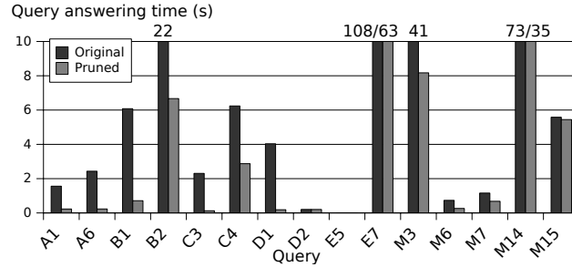
Fig. 9. Experimental results for the MonetDB engine
