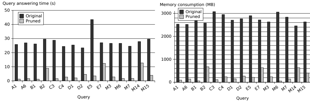
Fig. 8. Experimental results for the Saxon-b/XQuery engine
